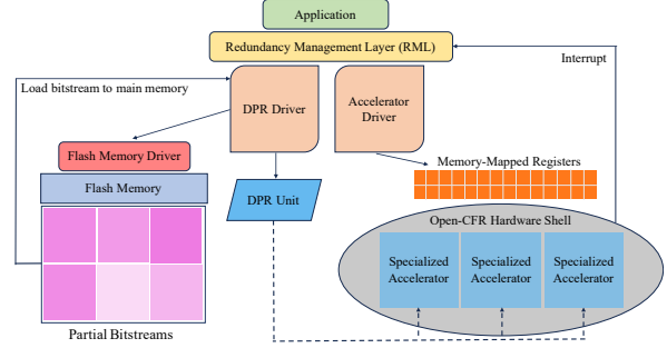
Fig. 3. The software architecture of the OPEN-CFR framework.
