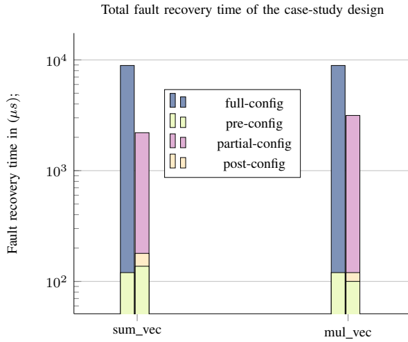
Fig. 8. Comparison of total fault recovery using a partial-reconfiguration vs full-reconfiguration approaches.
